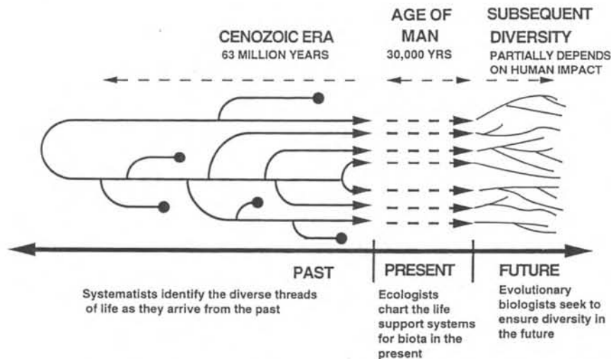
Fig. 1 The temporal framework for setting conservation priorities allocates responsibilities in three distinct temporal spheres (past, present, and future) to three disciplines (systematics, ecology, and evolution). The tree used here is based on the history of sea turtles inferred from molecular sequence comparisons (Bowen & Karl 1996; Dutton et al. 1996). The process of conserving sea turtles may start with the systematists identifying seven extant species which require protection. Subsequently, ecologists identify the key habitat features that allow sea turtles to survive and thrive on an ecological time-scale of a few tens of thousands of years. Finally, evolutionary biologists identify the raw materials for future prosperity and diversification.
